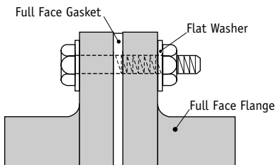
FULL FACE FLANGE CONNECTION
